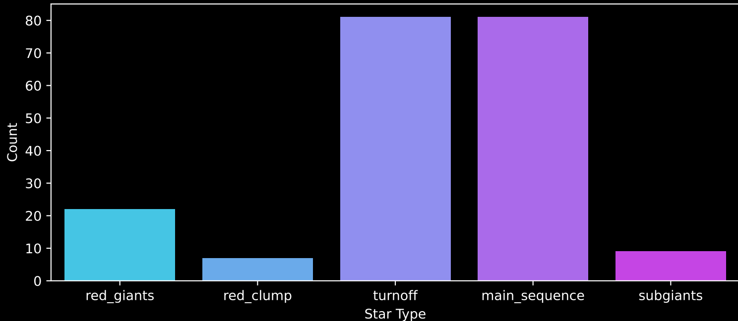
GALAH DR4 Field: [7216] Count plot of Star Type
