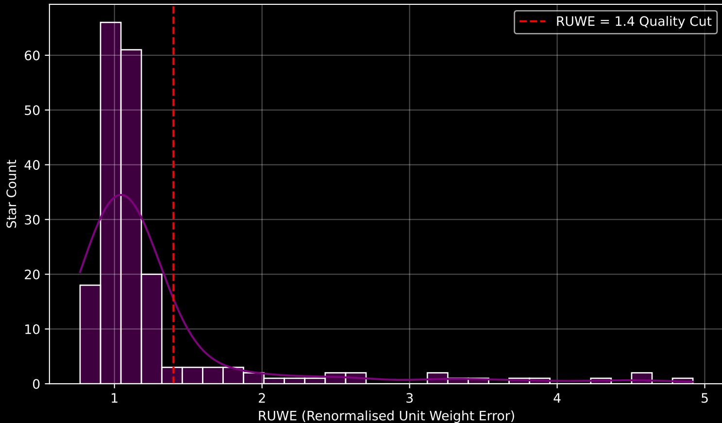
GALAH DR4 Field [7216] RUWE Distribution (n= 196)
