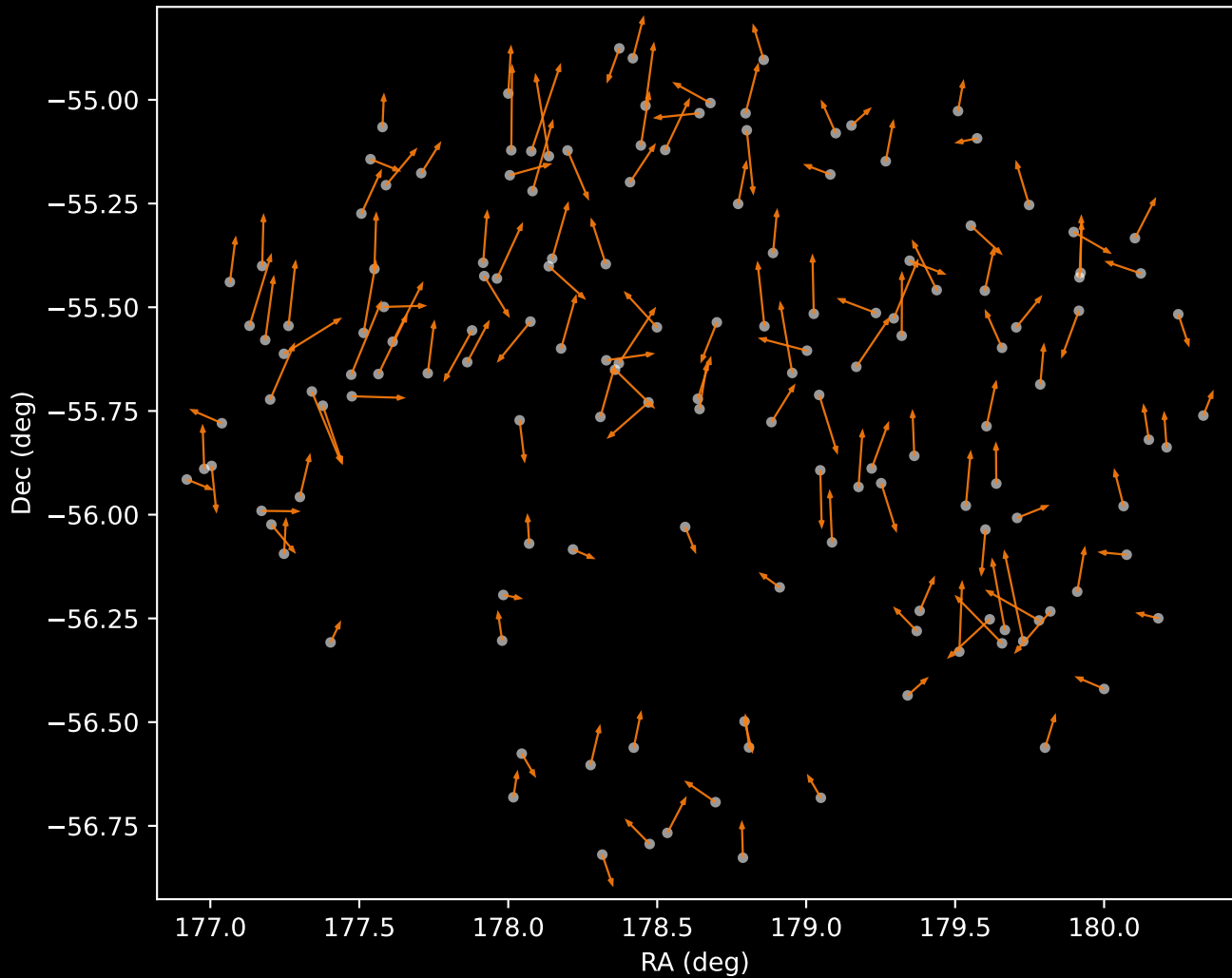
GALAH DR4 Cluster 2 Proper Motion Vectors (n=150)
