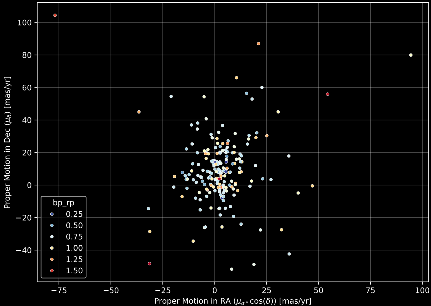
GALAH DR4 Field: [7216] Proper Motion Diagram (n= 200)
